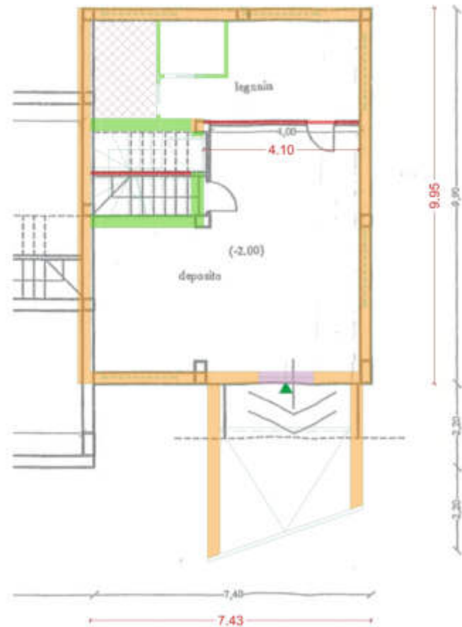
PIANO SEMINTERRATO
